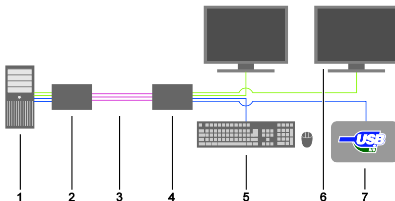
KVM Extender (Dual-Head with 4x USB-HID)
