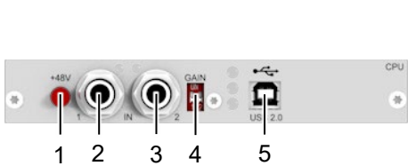
Fig. 30 Interface side L-/R474-BBE2
